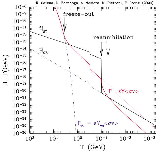
FIG. 8 (color online). The expansion rate of the Universe \tilde{H} and the WIMP interaction rate \Gamma = Ys\langle\sigma_{\text{ann}}v\rangle are plotted as a function of the temperature. The reannihilation effect discussed in the text is outlined. The small drop in the rates at T = 300 MeV is due to the quark-hadron phase transition.
