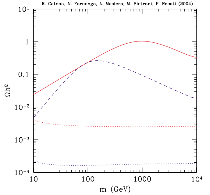
FIG. 13 (color online). The relic abundance in a ST theory as a function of the WIMP mass in the case of \langle \sigma_{\text{ann}} v \rangle \equiv a = 1 \times 10^{-7} GeV (solid line) and \langle \sigma_{\text{ann}} v \rangle \equiv b/x = 1 \times 10^{-4} GeV/x (dashed line). The upper (lower) dotted lines corresponds to the GR case for \langle \sigma_{\text{ann}} v \rangle \equiv a = 1 \times 10^{-7} GeV and \langle \sigma_{\text{ann}} v \rangle \equiv b/x = 1 \times 10^{-4} GeV/x, respectively.
